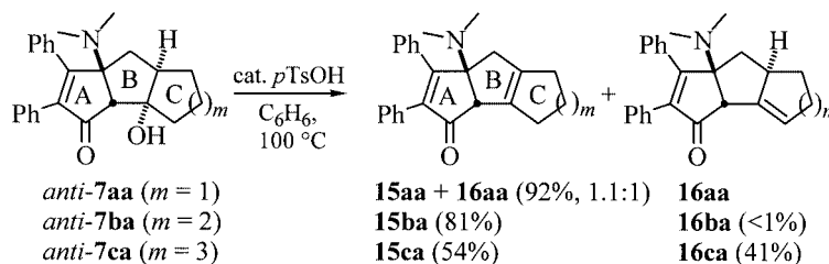
Scheme 4. Dehydration of tricyclic hydroxy ketones anti -7.
